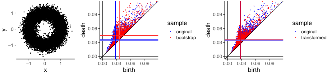
FIG 2. Left: The original data set of size n = 10,000 , from which a single standard bootstrap sample is drawn. Middle: Persistence diagrams for both the original and bootstrap samples, along with lines denoting the median birth and death in each diagram. The asymptotic bias discussed in Section 4.1 can be clearly seen. Right: Persistence diagrams after application of a multiplicative correction factor of \sqrt{1 - e^{-1}} \approx 0.795 to the bootstrap sample. Note that the median birth and death values correspond after this transformation is applied.
